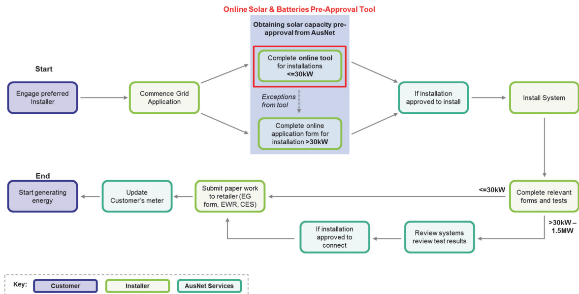
Figure 5: Diagram of process for embedded generator connections
